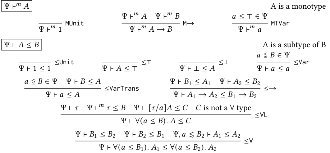
Fig. 2. Declarative Monotype and Subtyping
